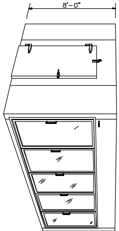
PERSPECTIVE VIEW
