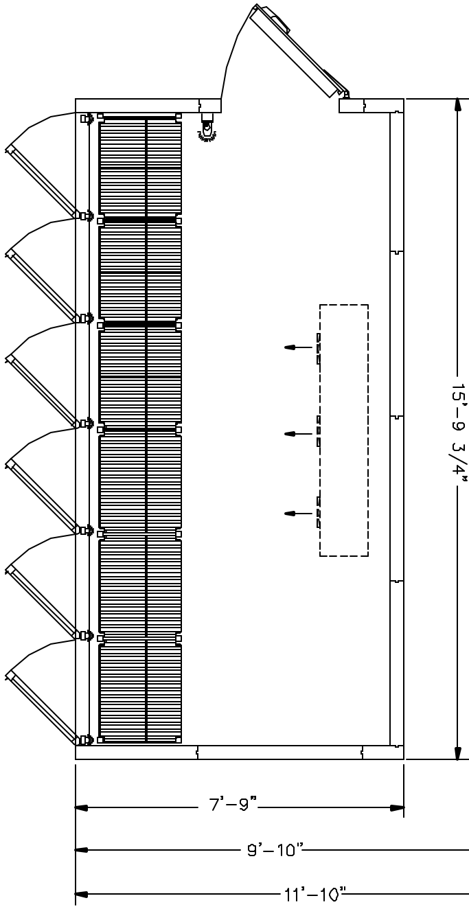
PLAN VIEW
