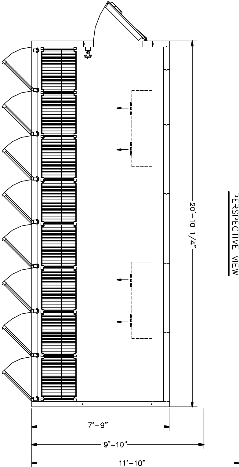
PLAN VIEW
