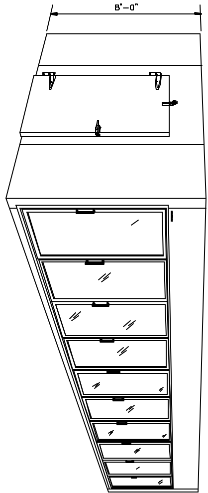
PERSPECTIVE VIEW
