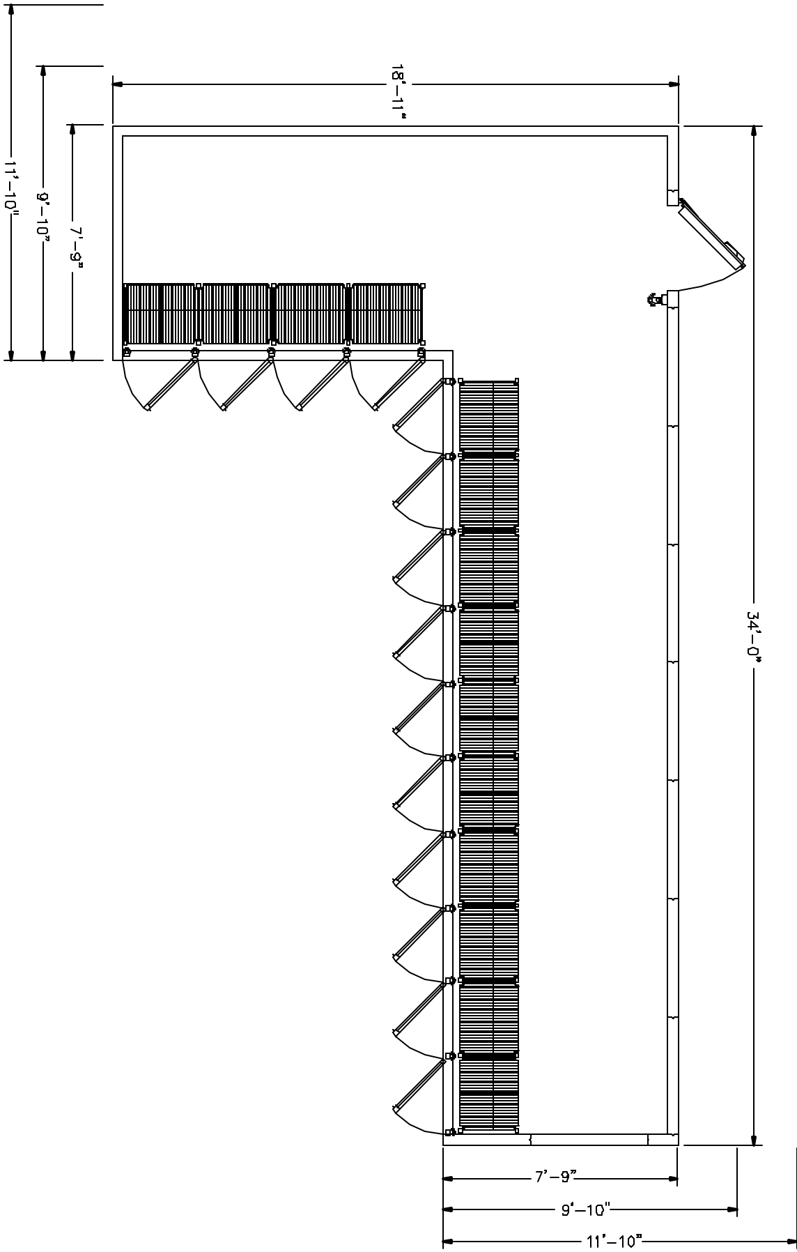
PLAN VIEW
