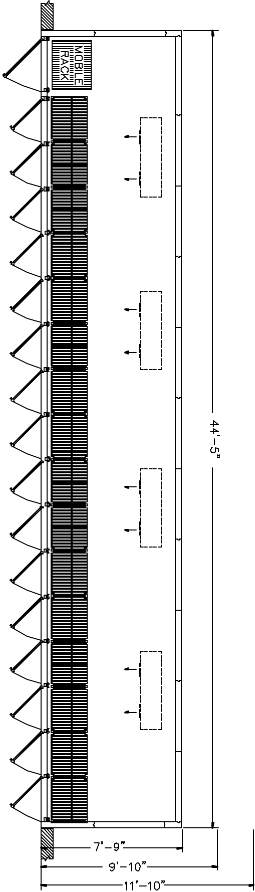
PLAN VIEW
