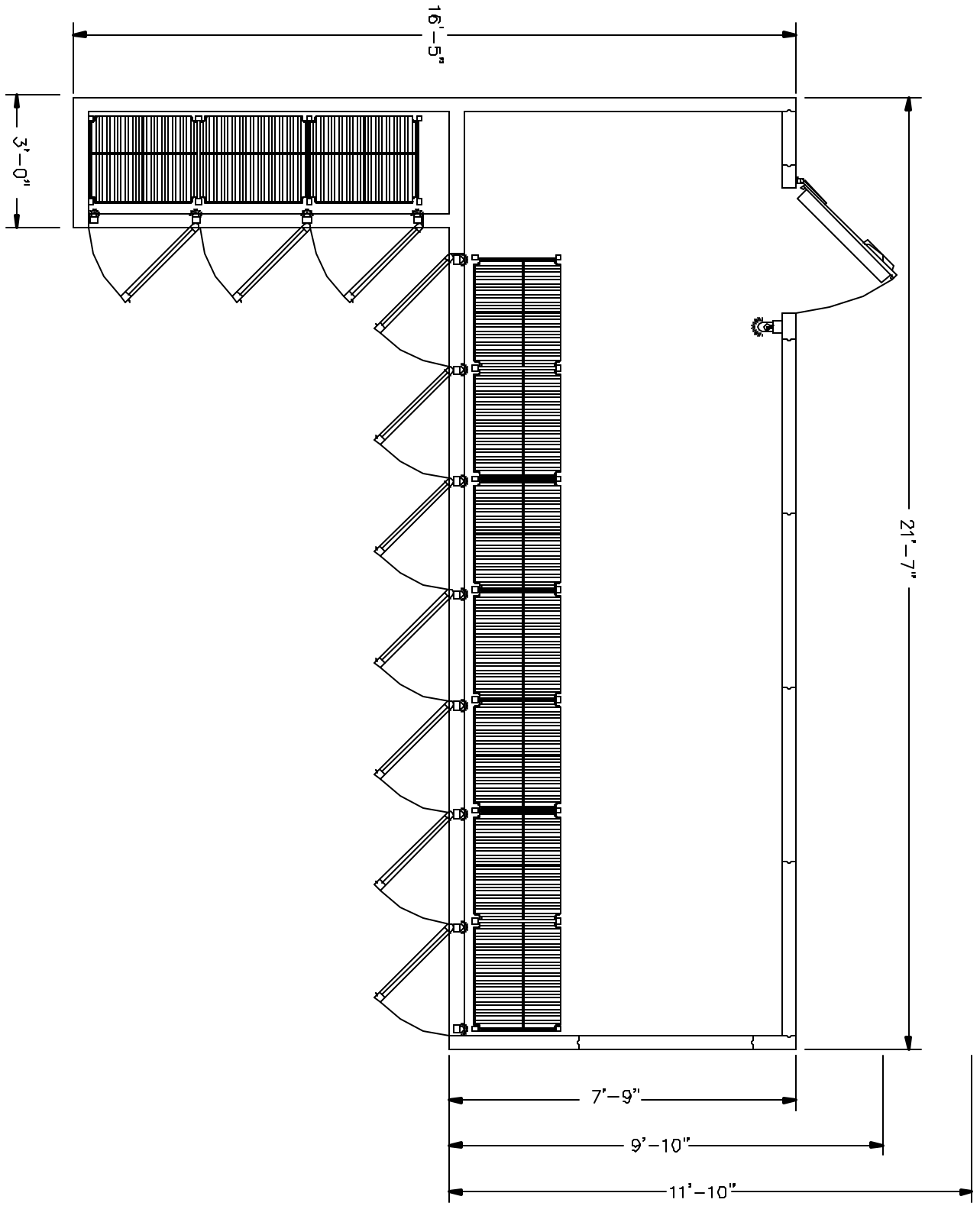
PLAN VIEW
