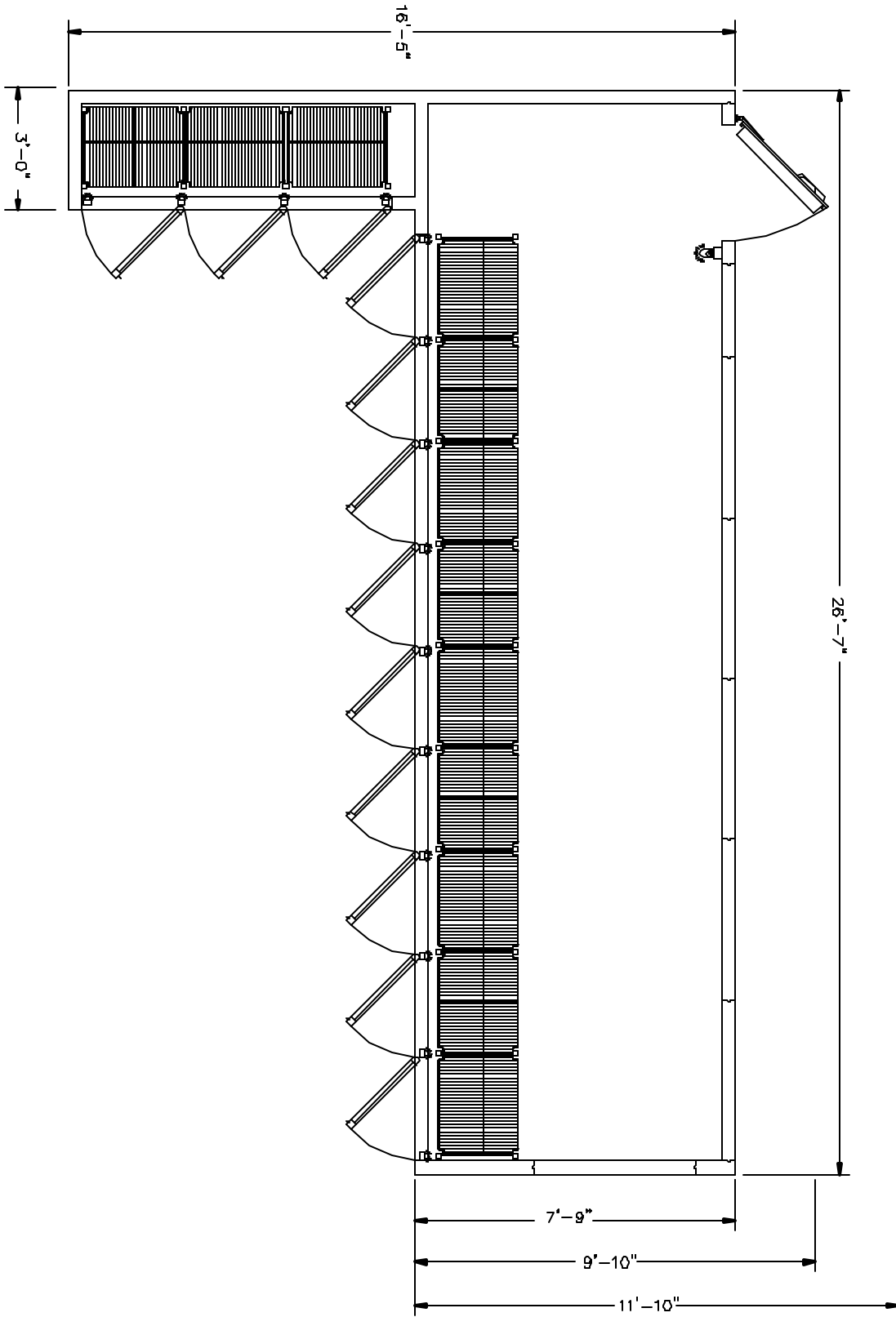
PLAN VIEW
